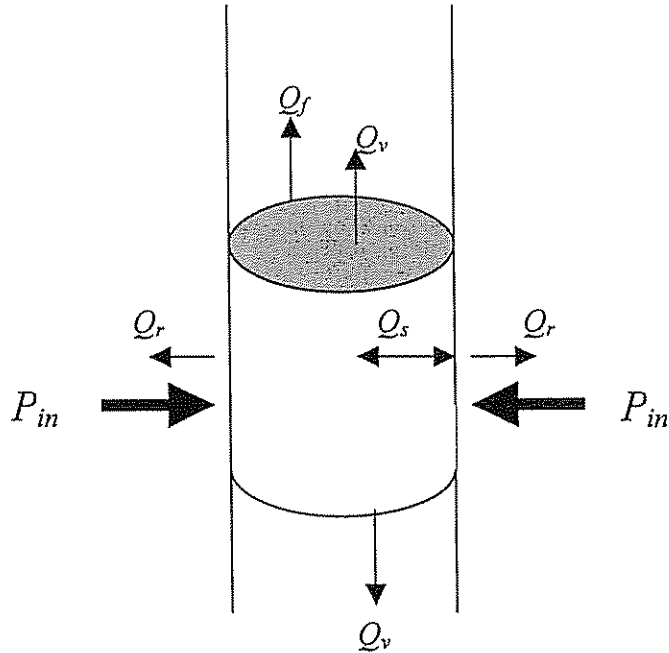
Figure 2 The constant power stem heat balance principle: different forms of heat loss Q_r , Q_s and Q_v are in balance with electrical power supplied to the heater P_{in} . Source: Adapted from Smith and Allen (1996).
