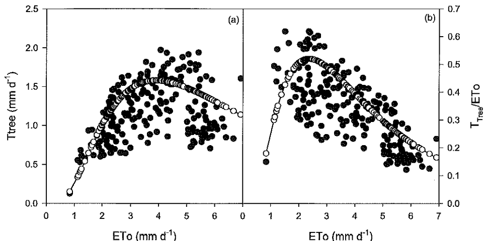
Figure 3. Relationships between reference evapotranspiration ( E_{To} ) and (a) daily transpiration ( T ) and (b) the ratio T/E_{To} of I. densiflora in an agroforestry system at San Pedro de Barva, Costa Rica.
