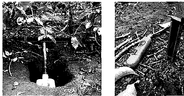
Photography 8. Detailed views of the measurements of water runoff (a) and soil water content with TDR (b) on the research station of CICAPE, San Pedro de Barva, Heredia, Costa Rica.
