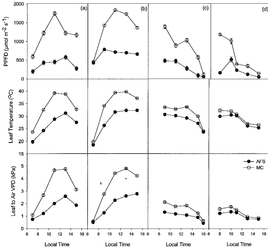
Figure 18. The diurnal time course of PPFD, leaf temperature and leaf to air VPD of coffee leaves during the dry season (a: February; b: March 2005) and the wet season (c: August; d: September 2005) in MC and AFS at San Pedro de Barva, Costa Rica. (Values are averages of 4 leaves in 4 plants measured over a period of 1 hour).
