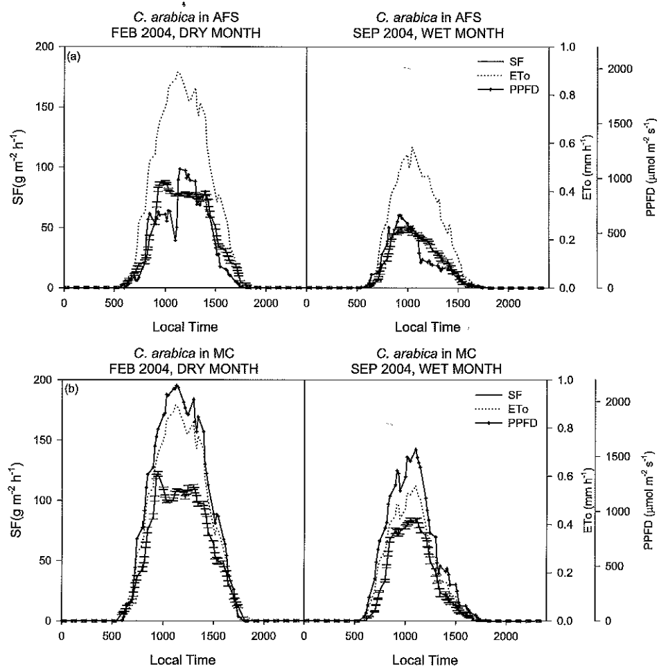
Figure 4. Mean hourly coffee sap flow rate (SF), reference evapotranspiration ( E_{To} ; measured in open field) and photosynthetic photon flux density (PPFD) based on ten consecutive days and four coffee plants in AFS (a) or in MC (b) for a dry month (February) and wet month (September) in San Pedro de Barva, Costa Rica (values \pm sd are means over periods of 15 min).
