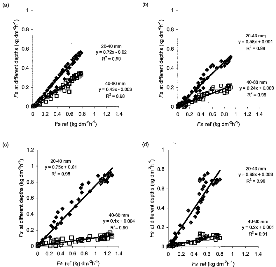
Figure 2. Relationships between values of sap flow at depths of 20-40mm and 40-60mm and the outer depth of 0-20mm during monitoring periods of 15 minutes over 15 days.
