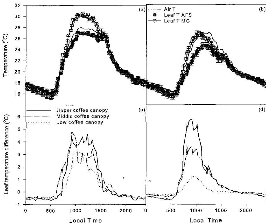
Figure 7. Mean diurnal leaf temperature (ab) and mean diurnal differences in leaf temperature (cd) at different coffee canopy strata between monoculture and an agroforestry system shaded with Inga densiflora in San Pedro de Barva, Costa Rica, for April 2005 (dry season, left panels) and July 2005 (rainy season, right panels).
