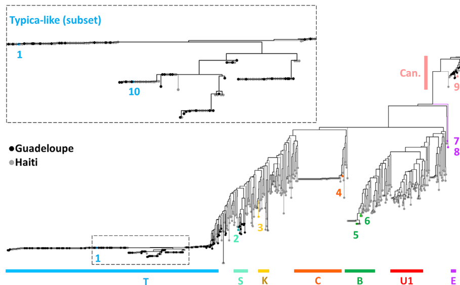
FIGURE 3 Unweighted neighbor-joining dendrogram of Guadeloupe (in black), Haitian (in gray) and reference (in color) C. arabica and C. canephora individuals. Calculated from simple-matching distance matrix. Colored bars represent varietal groups identified by sNMF population structure analysis: C = CR95/Catimor-like, K = Kent/l60-like, T = Typica-like, B = Bourbon-like, E = Ethiopian-like, S = SL/Kenyan-like, U1 = Unlabeled1 (Haiti-only) group, plus Can. = Canephora outgroups. A portion of the Typica branch is magnified (in frame). To aid legibility, a few representative reference individuals are included, colored according to their assigned varietal group (excluding Canephora) as identified by sNMF population structure analysis. These are as follows: 1. (Ku214) Typica/Jamaica Blue Mountain, 2. (T.04313) SL28, 3. (T.04268) Kent, 4. (T.08667) CR95, 5. (Mw264) PR6791/Bourbon Select, 6. (T.02542) Caturra, 7. (T.04667) E-160, 8. (T.04290) Jimma Kaffa, 9. (GUI2) Guinean C. canephora , and 10. (T.00990) Surinam.
